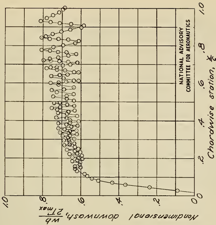
Figure 5. - Chordwise distribution of the nondimensional downwash wb/2\Gamma_{max} at \frac{y}{b/2} = 0 and \frac{z}{b/2} = 0.011 . Flat-plate type of loading.
